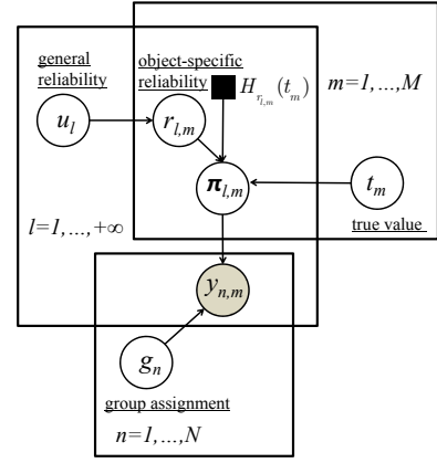
Figure 2: The graphical model for multi-source sensing. The three plates represent group reliability u_l with l = 1, 2, \dots , the true values t_m for each object O_m with m = 1, \dots, M , and the group assignment g_n of each source with n = 1, \dots, N , respectively.
